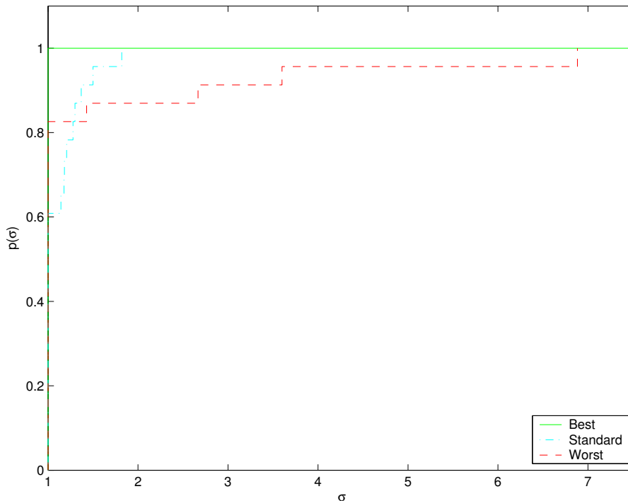
Figure 4.5: CPU time performance profiles for the best, standard and worst parameter choices
