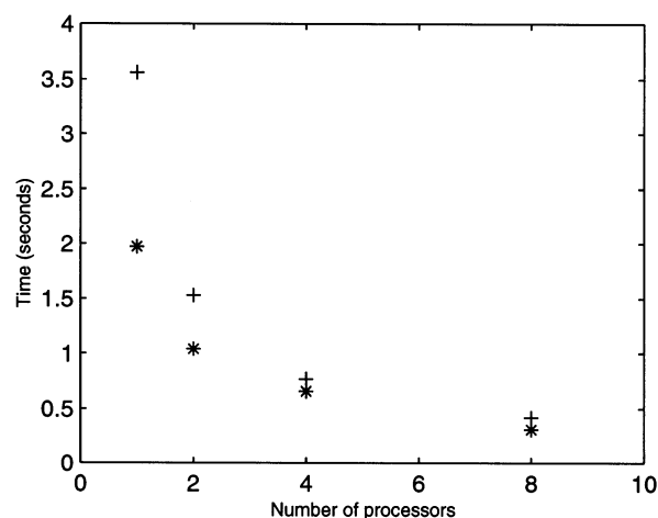
Fig. 4. Factorization times for bayer01 (*) and icomp (+) on one, two, four, and eight processors.
