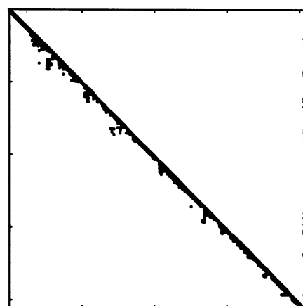
Fig. 3. Problem bayer04 after reordering with MSRO(3, W_3 ).
