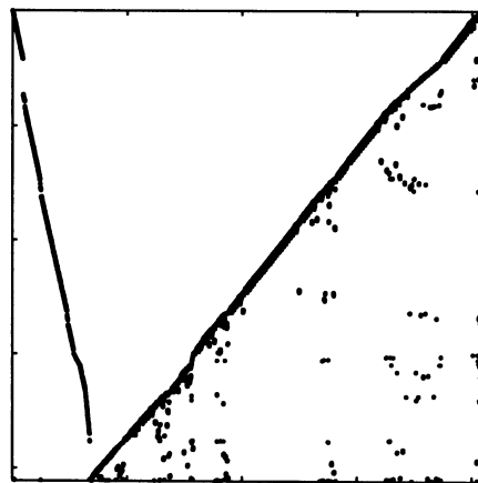
Fig. 1. Problem bayer04 with original ordering.
