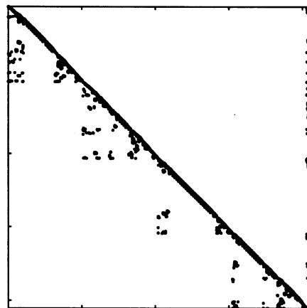
Fig. 2. Problem bayer04 in bordered block diagonal form.
